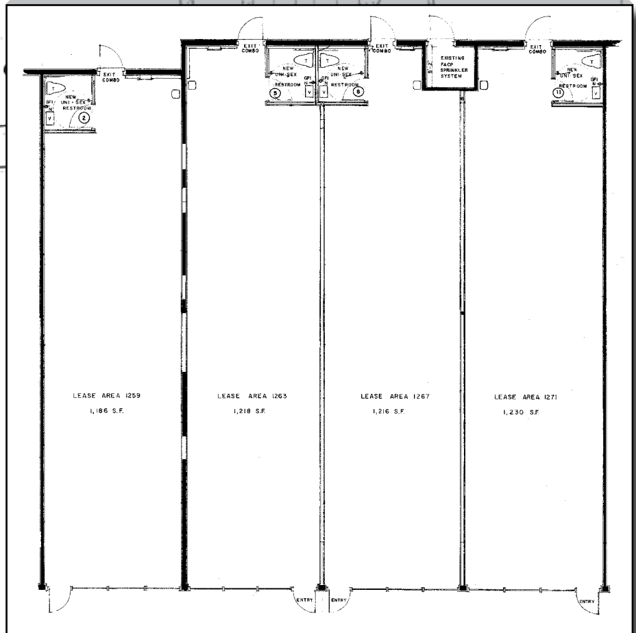
SITE PLAN LAKE KAHRYN PLAZA
